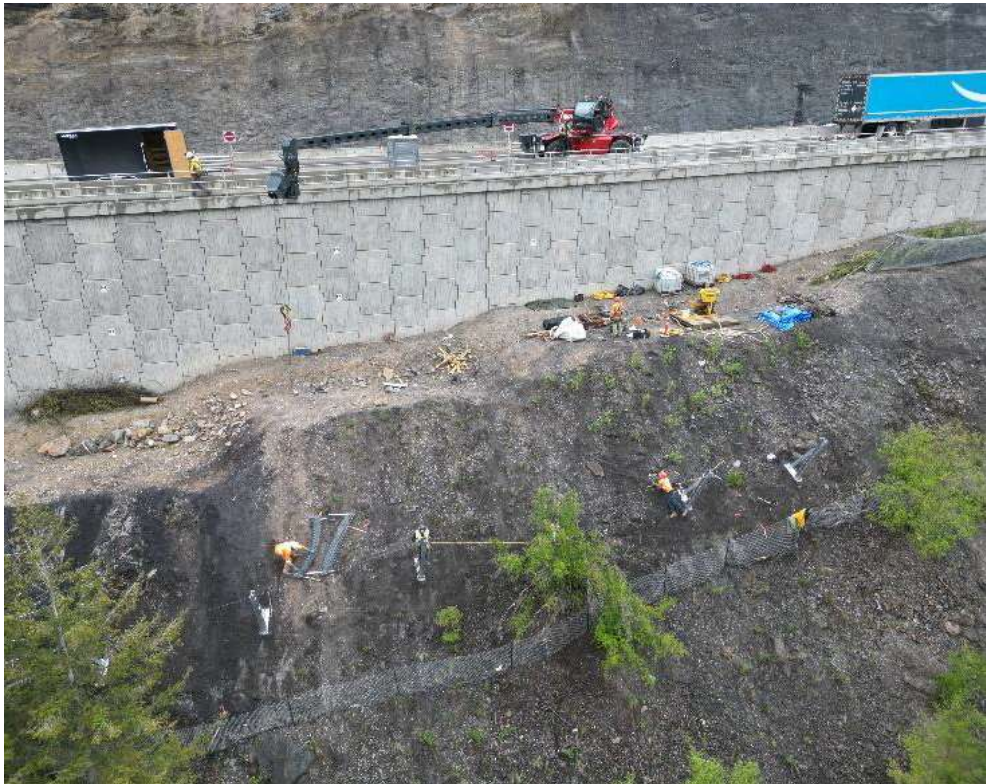
Figure 4: Snow protection fence installation downslope from Grizzly Viaduct – May 16, 2024
